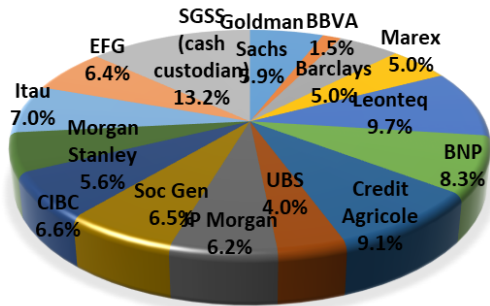
Counterparty exposure
